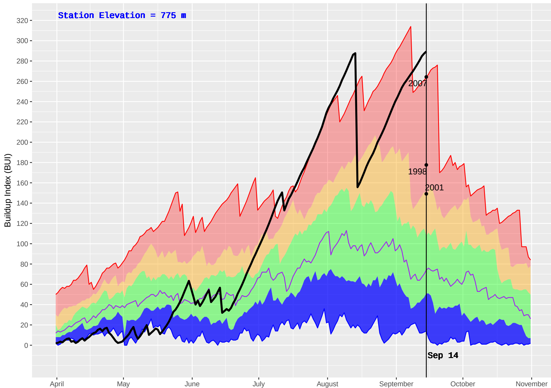
ELKO (412) : Historical (1970–2016) and Current (2017) Noon Buildup Index (BUI)
