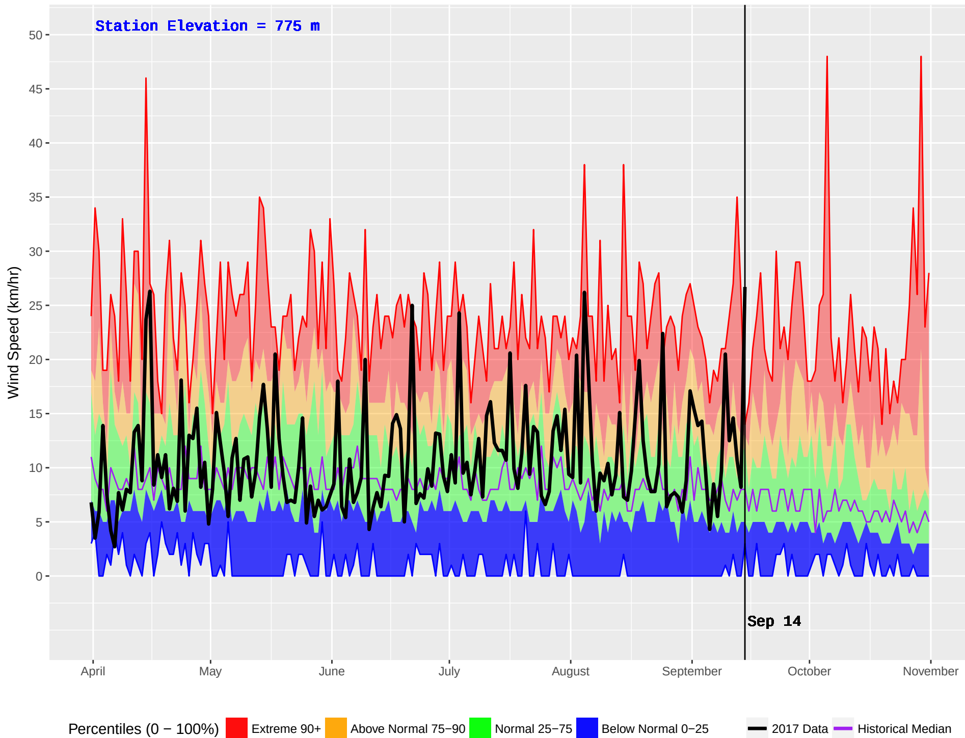
ELKO (412) : Historical (1970–2016) and Current (2017) Noon Wind Speed
